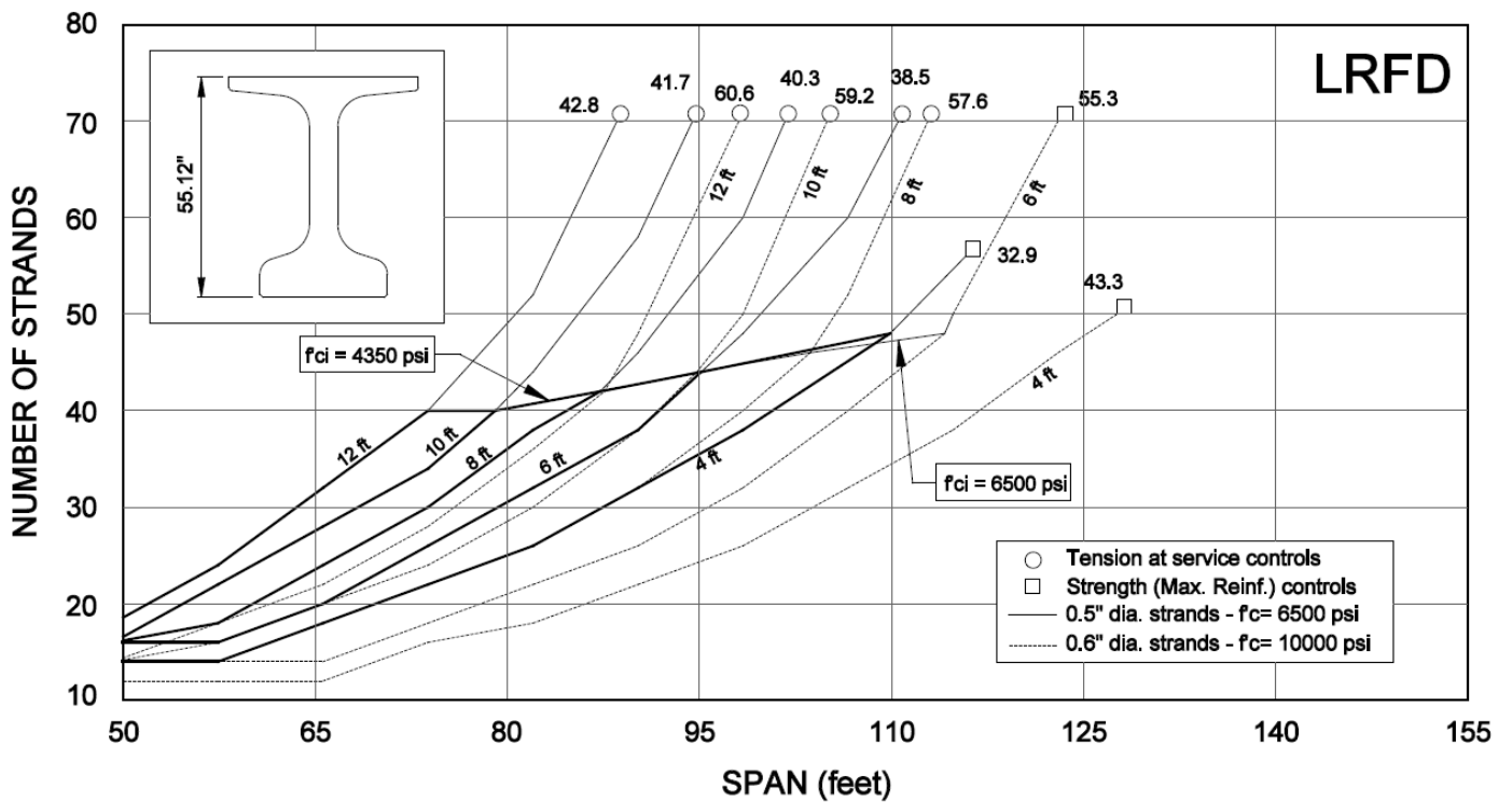
Chart NEBT-16 Northeast Bulb-Tee - NEBT 55
