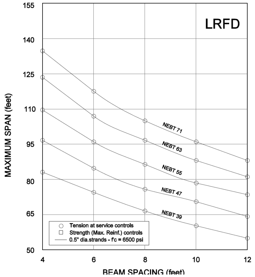
Chart NEBT-13 Northeast Bulb-Tee
