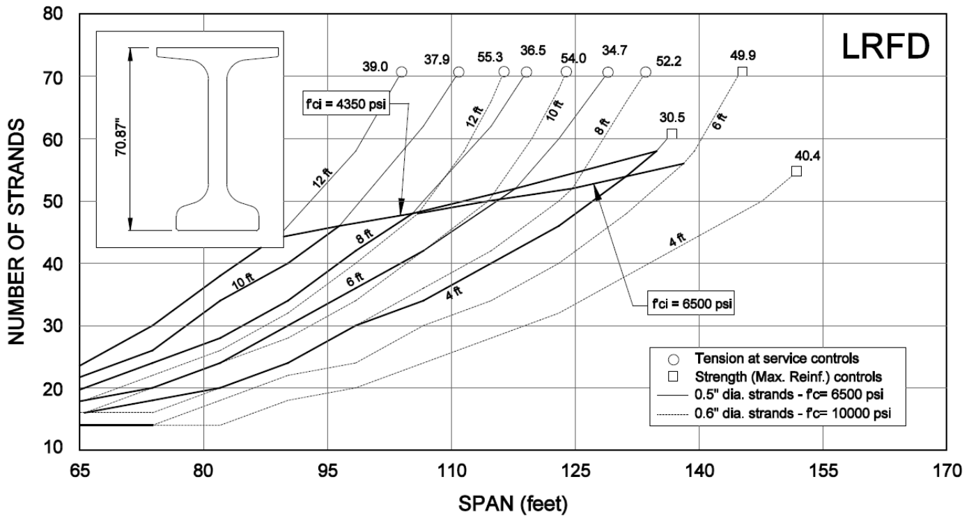
Chart NEBT-18 Northeast Bulb-Tee - NEBT 71
