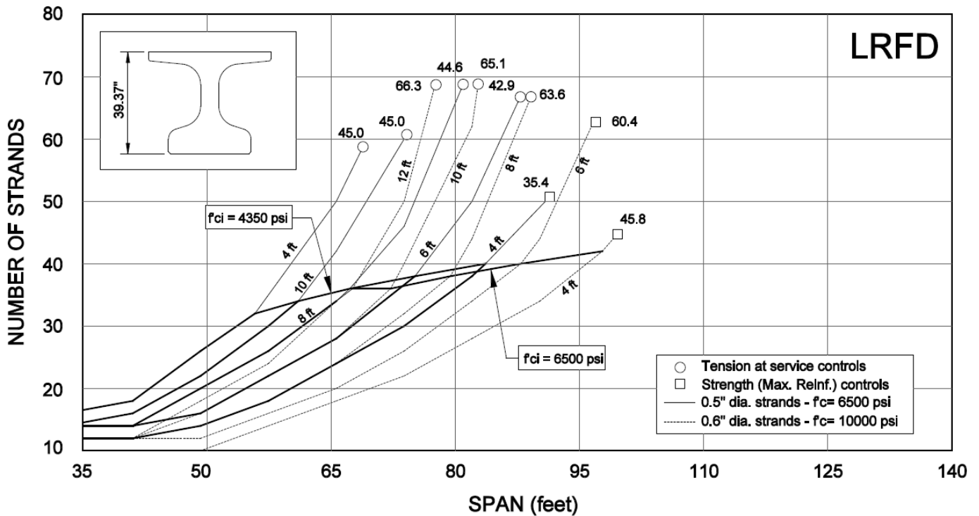
Chart NEBT-14 Northeast Bulb-Tee - NEBT 39
