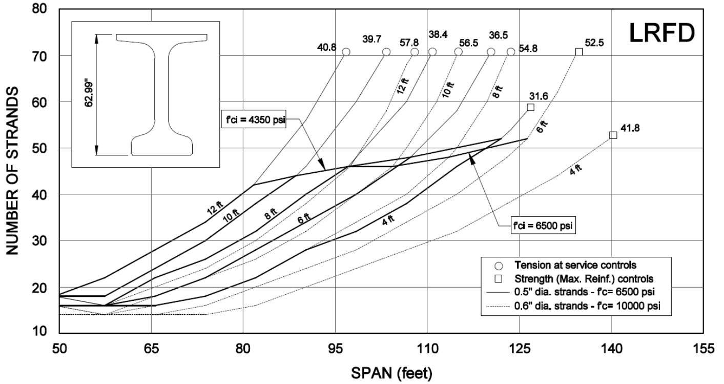
Chart NEBT-17 Northeast Bulb-Tee - NEBT 63
