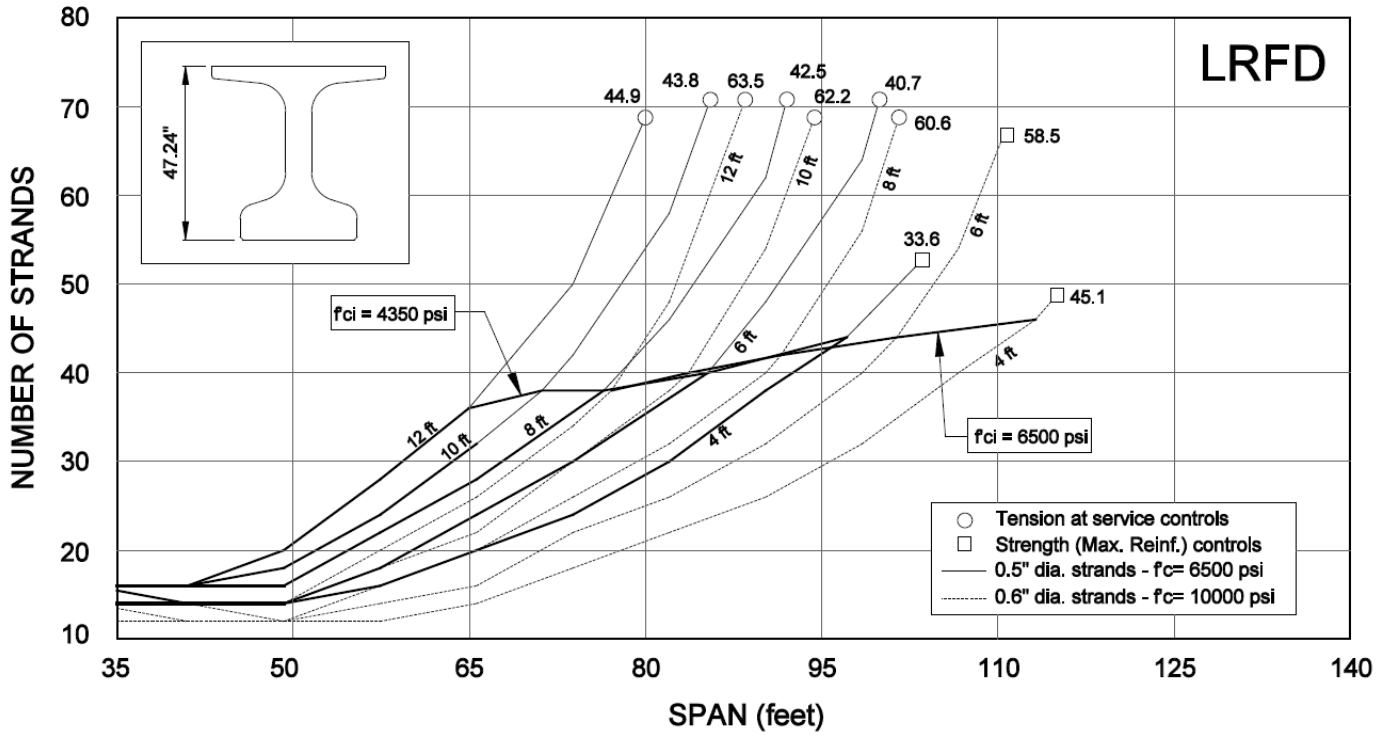
Chart NEBT-15 Northeast Bulb-Tee - NEBT 47
